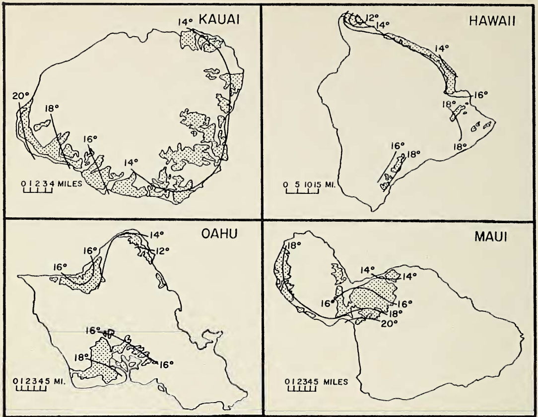
FIG. 7. Annual mean daily temperature range ( ^{\circ} F) in Hawaii.
